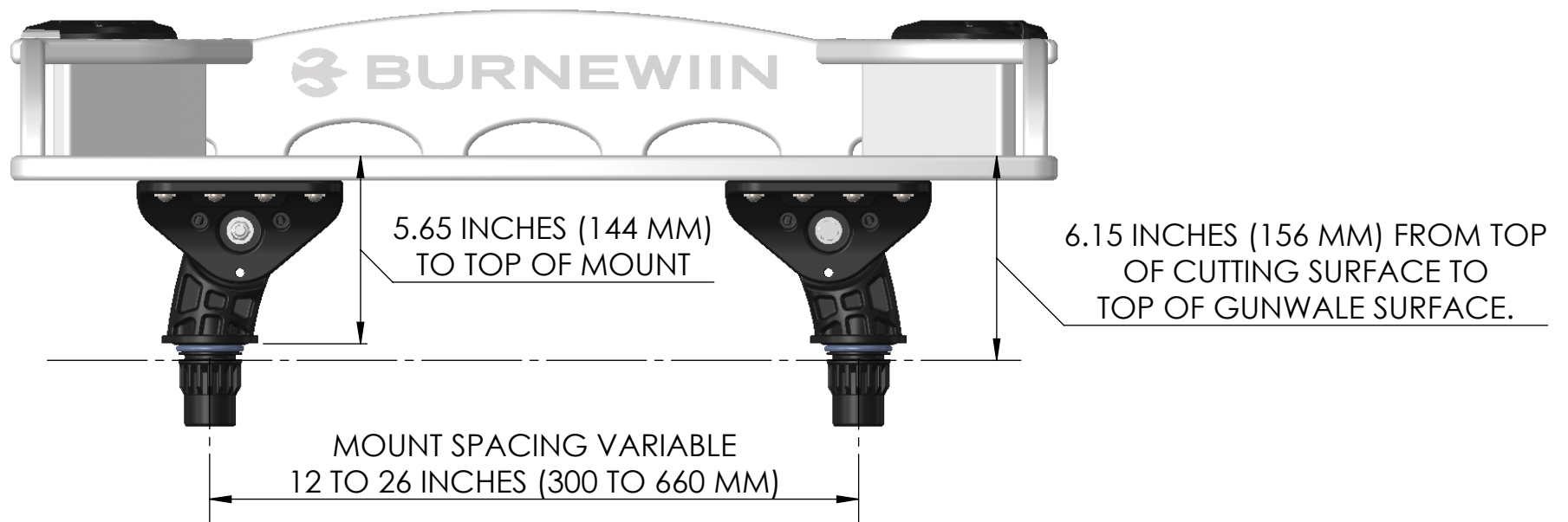
CB5315 MOUNTING DIMENSIONS
