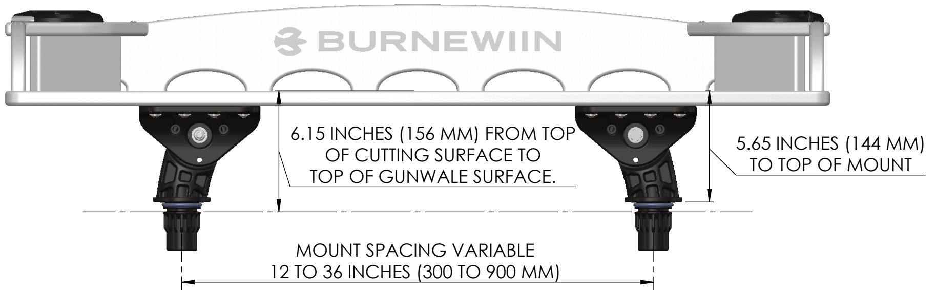
CB5420 MOUNTING DIMENSIONS
